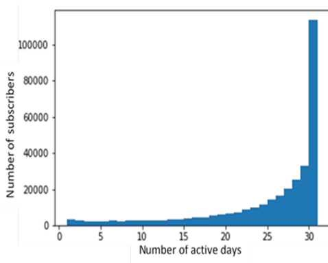
Fig. 7. Histogram of active days within a month
