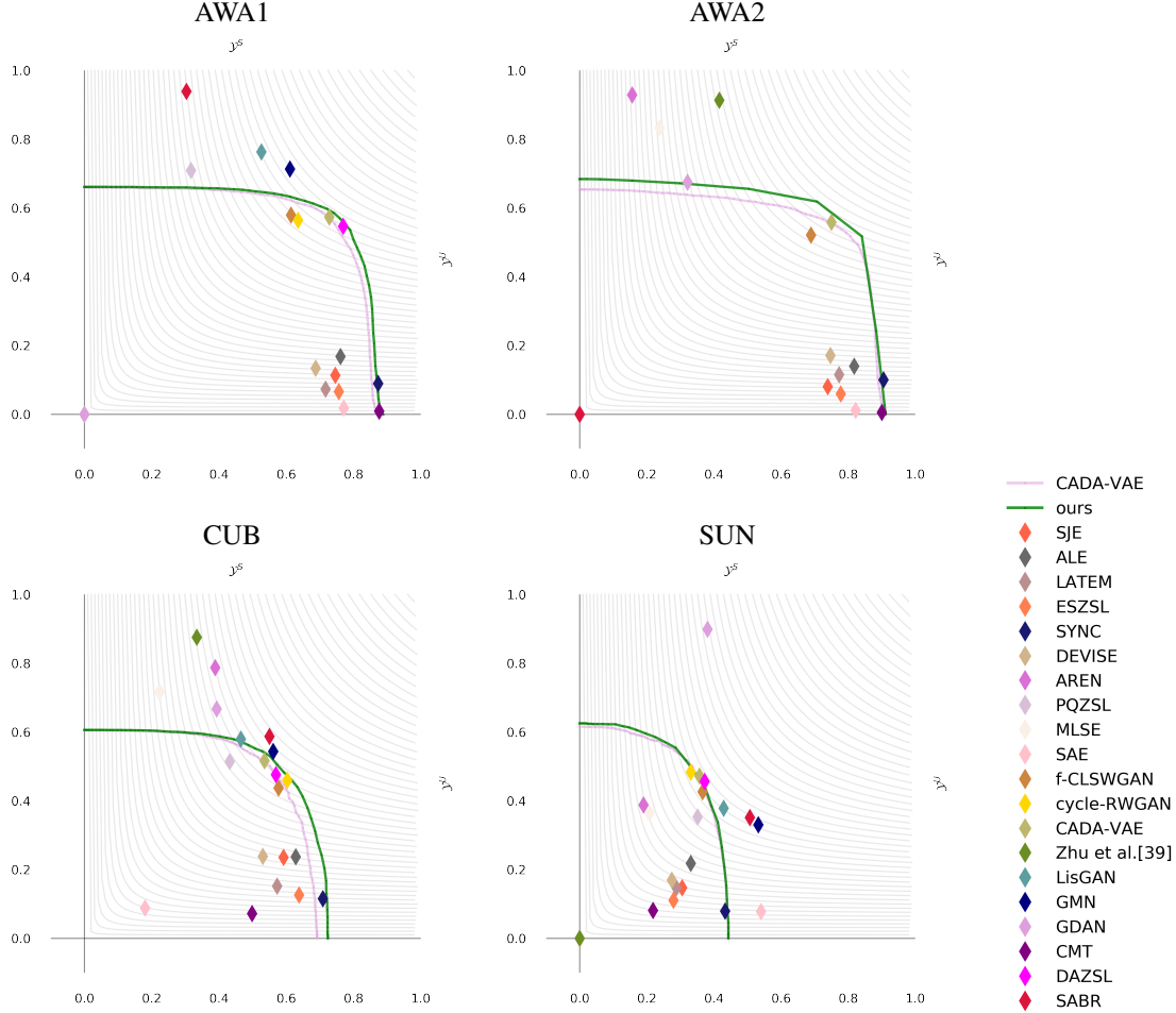
Fig. 2. The area for seen and unseen accuracy curve for the proposed method (green) and CADA-VAE [8] (pink), which is the closest model to ours (please see text and Table III for details about the methods). Note that these graphs are used to compute the AUSUC in Table II
