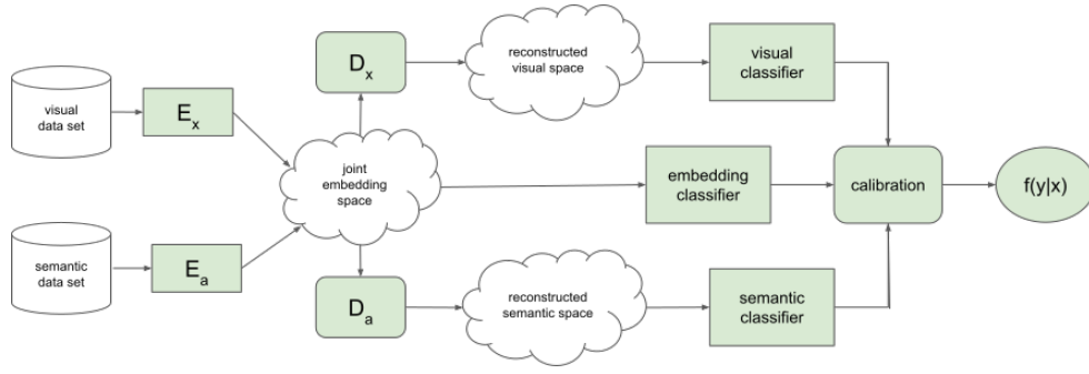
Fig. 1. Our model consists of encoders from visual and semantic spaces to a latent joint embedding space. Samples from the joint space are used to train decoders that reconstruct the original samples from visual and semantic spaces. Samples from the visual, semantic and joint spaces are then used to train and calibrate classifiers for each space. The final multi-domain classifier averages the results of the multi-modal calibrated classifiers.
